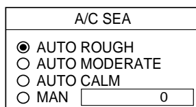
A/C SEA window
